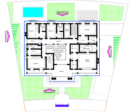
Second Floor Plan A = 312,66 m 2
