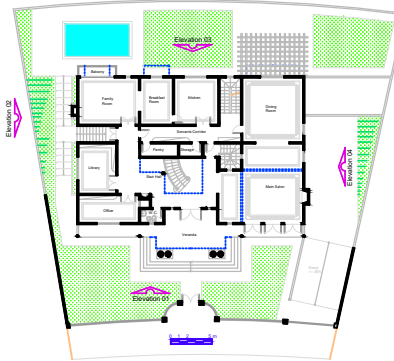
First Floor Plan A = 333,42 m 2
