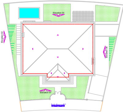
Roof Plan
